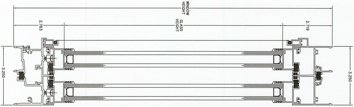
SECTION 2 SILL
